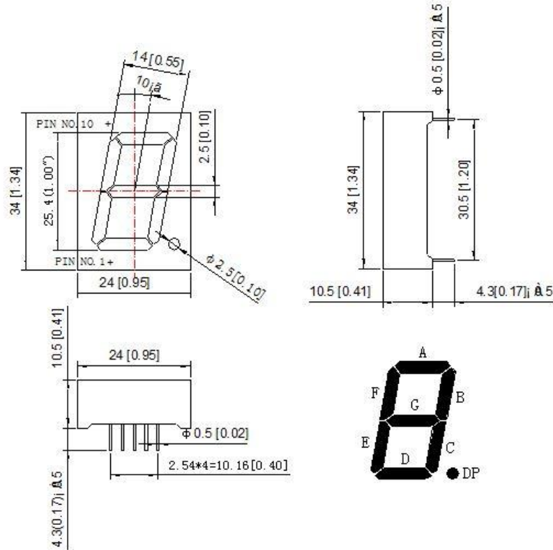
Common Anode
