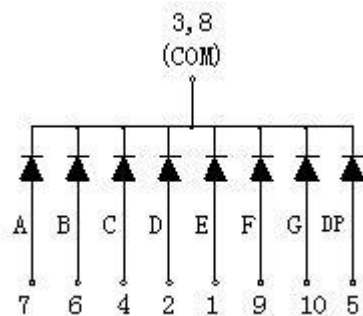
Common Cathode
