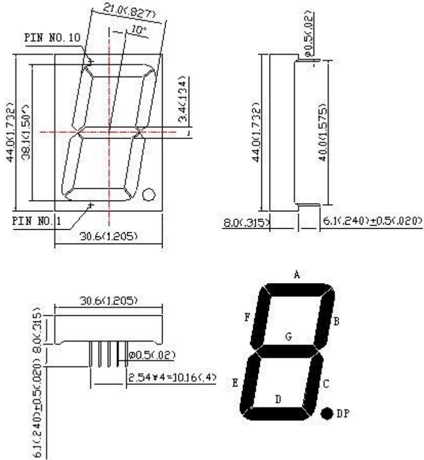
Common Anode
