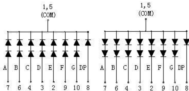
Common Anode
