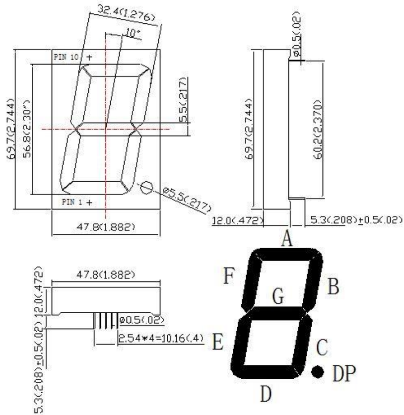
Common Anode
