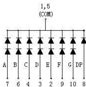
Common Anode
