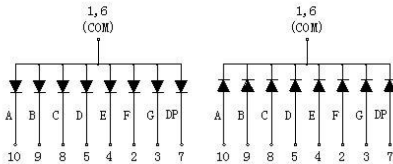
Common Anode
