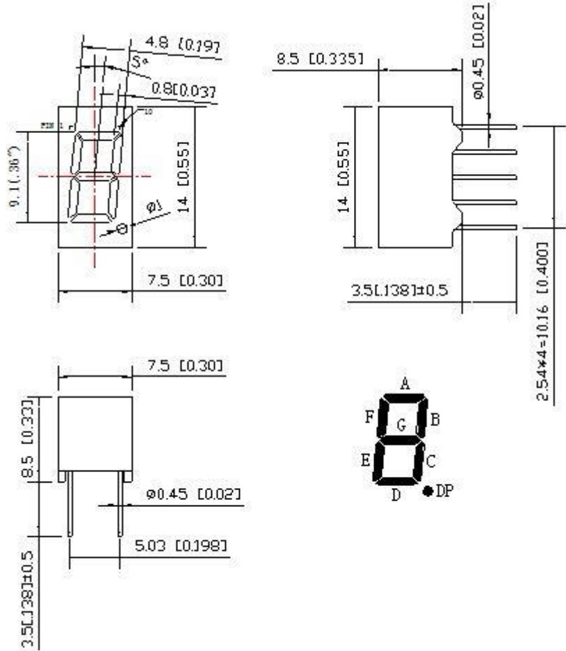
Common Anode
