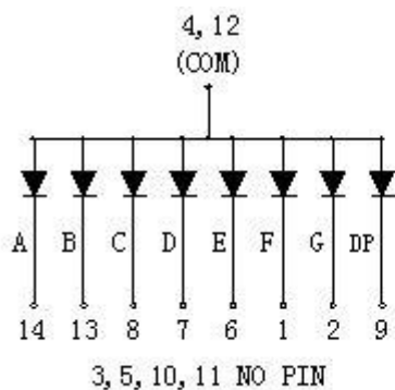
Common Anode
