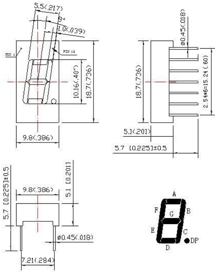
Common Anode
