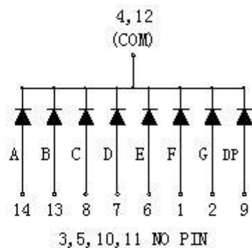
Common Cathode
