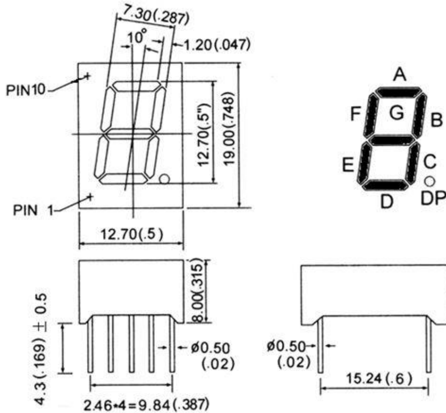
Common Anode
