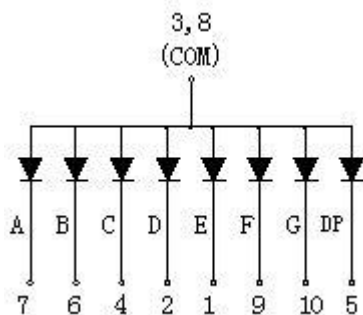
Common Anode
