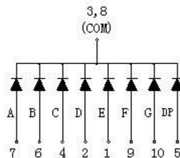
Common Cathode
