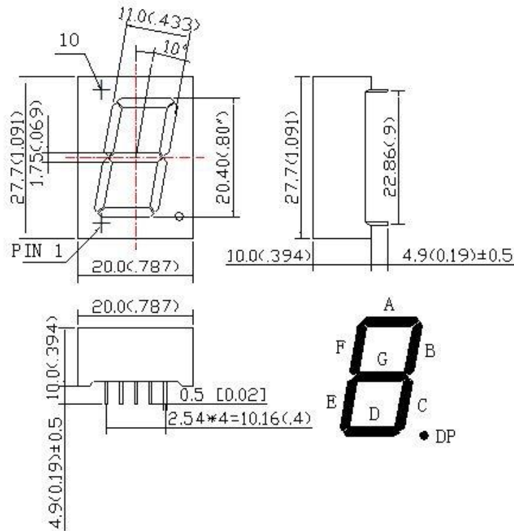
Common Anode
