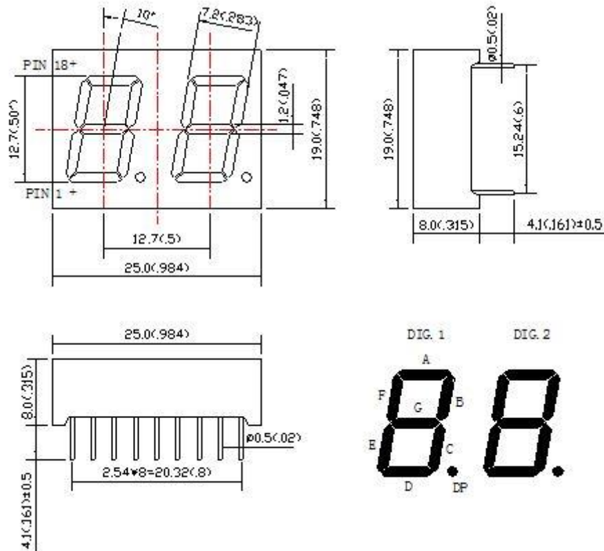
Common Anode
